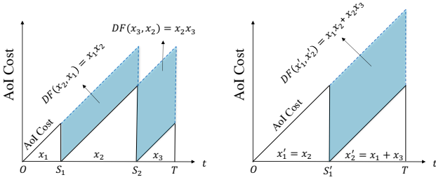
Fig. 5. Illustrations of Example 1 with a linear cost function. Combining the first interval into the third interval maintains the payment.
