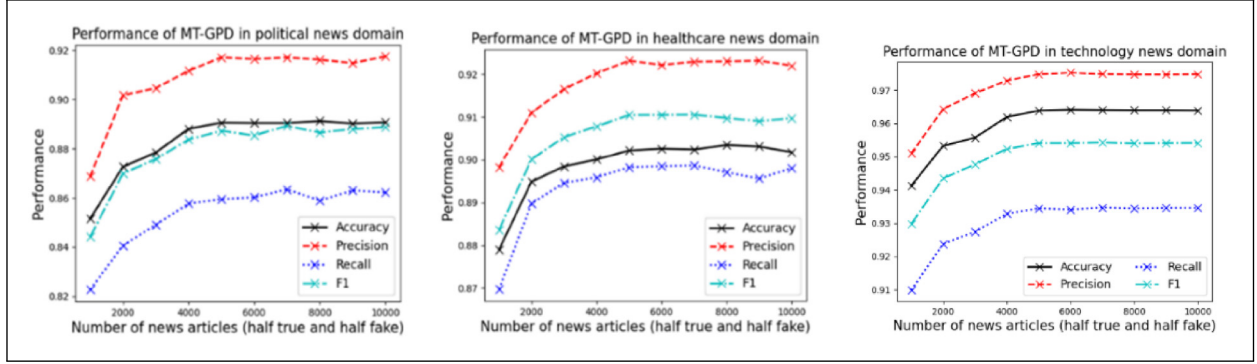
Figure 6. Results of sensitivity analysis on the impact of source-domain data size on MT-GPD performance.
