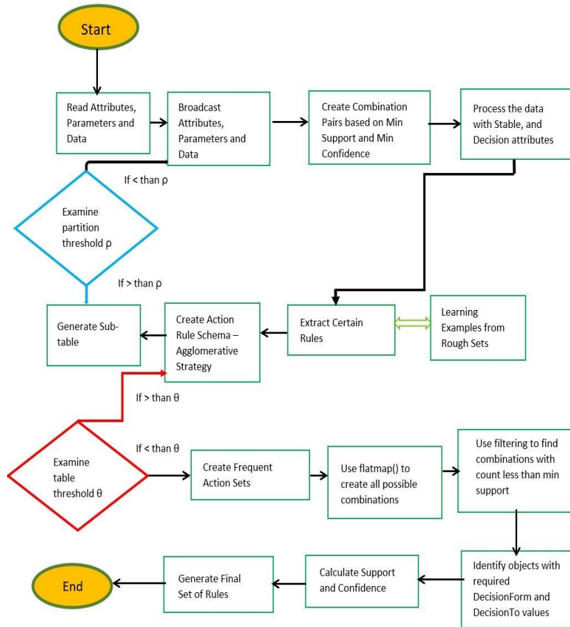
Fig.4. Hybrid Action Rule Mining Algorithm( New Threshold) - Flowchart.
