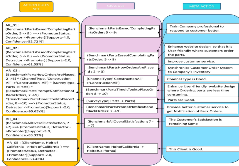
Fig.7. Example Meta Action for Table 8 From Action Rule 1 - To Action Rule 5
