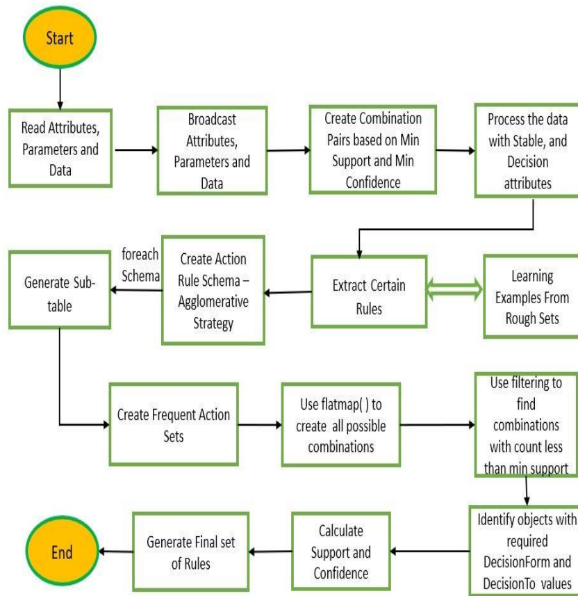
Fig.3. Hybrid Action Rule Mining Algorithm - Flowchart.
