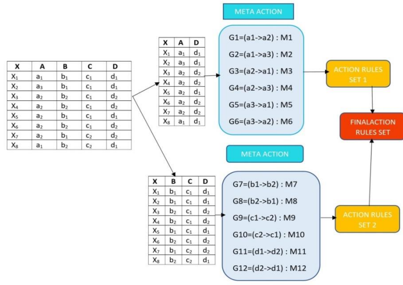
Fig.6. Vertical Data Split with Meta Action for Table 1
