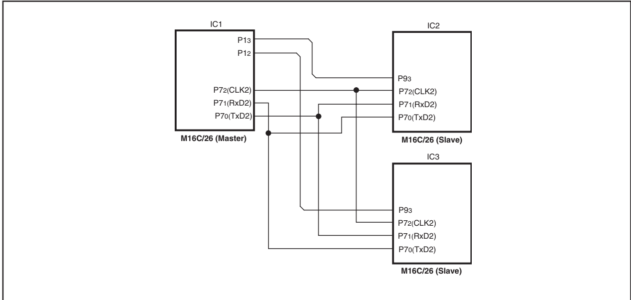
Figure 1.15.32. Programmable serial bus communication control example
