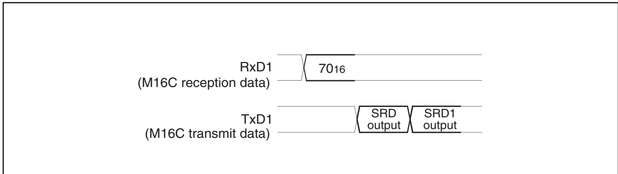
Figure 1.23.3. Timing for reading the status register
