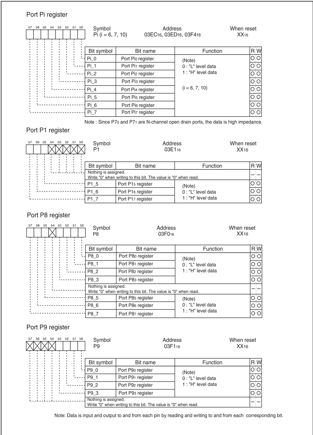
Figure 1.17.6. Port registers
