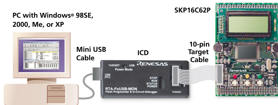
Figure 2. SKP16C62P System Connectivity
