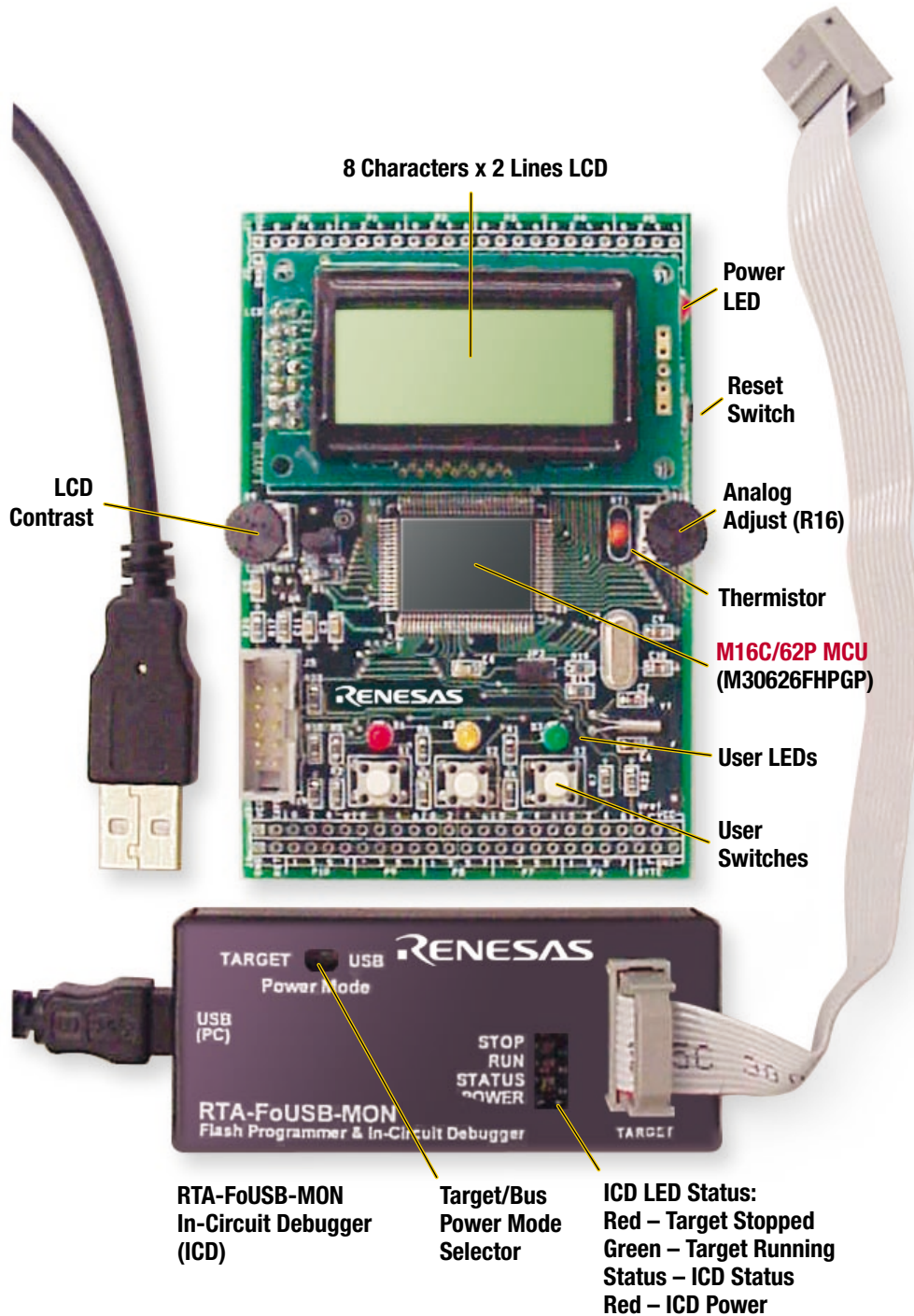
Figure 1. SKP16C62P
