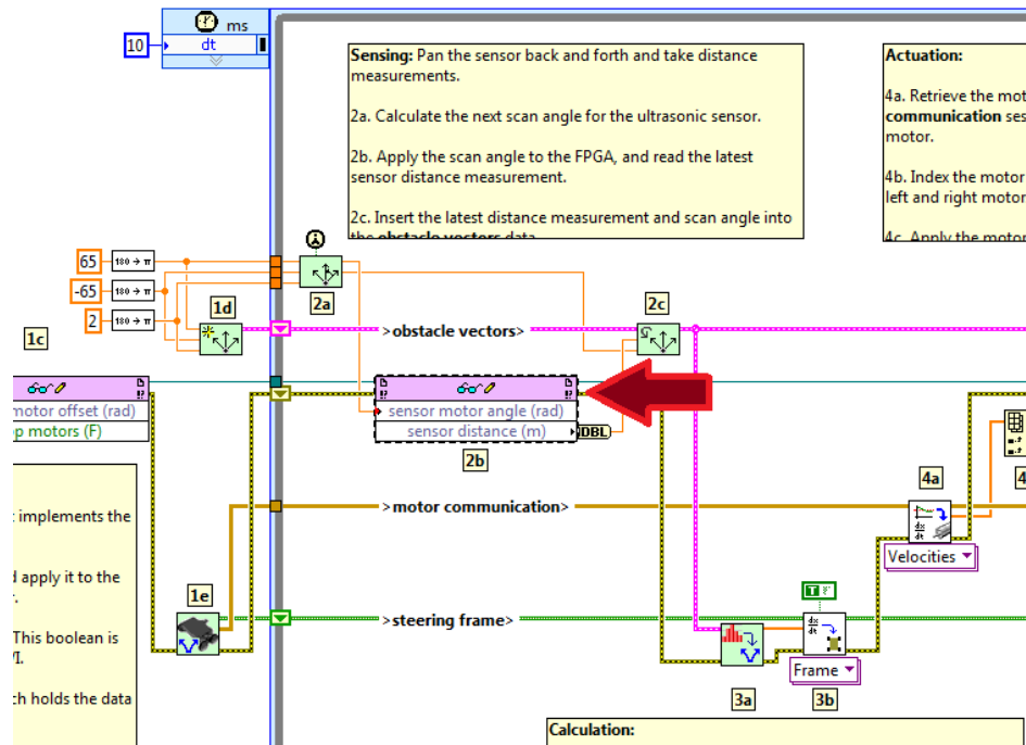
Figure 2.4 Exert From Roaming.vi
