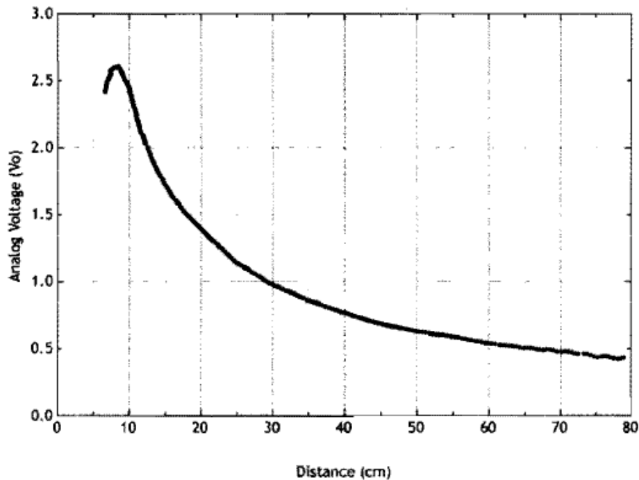
Figure 2.3: Analog Output vs. Distance to Reflective Object [2]
