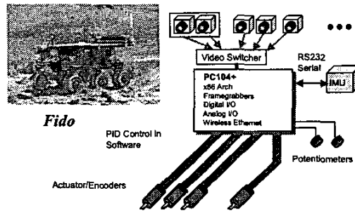
Figure 5: Centralized memory-mapped motion control architecture for FIDO
