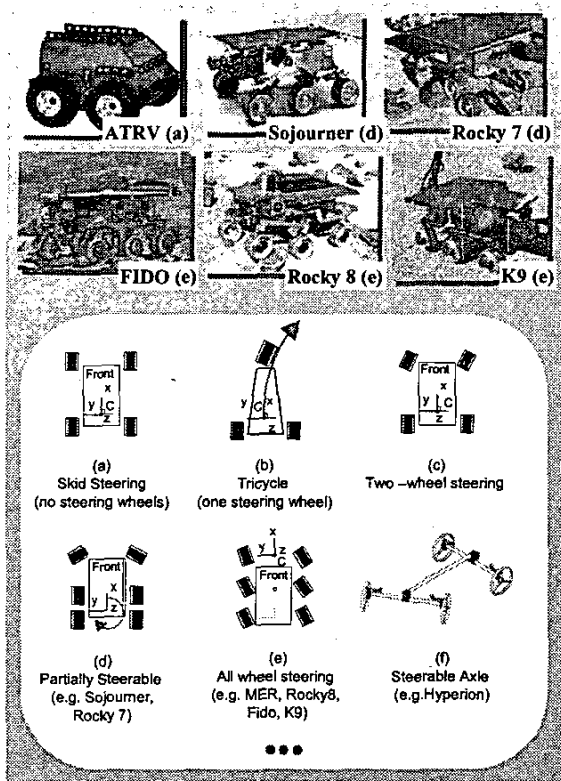
Figure 2: Various types of wheeled locomotors
