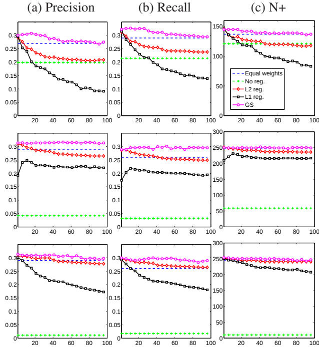
Figure 4. Annotation results of different regularization methods. 1st row: Corel5K; 2nd row: IAPR TC12; 3rd row: using weights calculated from Corel5K to test IAPR TC12. The legend is shown in the third figure of the first row. The horizontal axis represents the tuning parameter \lambda , from 1 to 100 with step size 5. The vertical axis represents the performance such as precision and recall.
