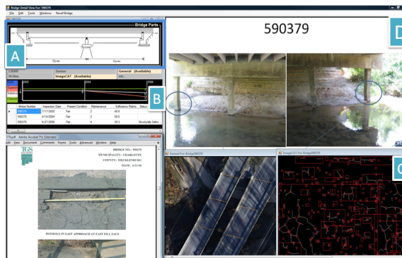
Figure 2: The Detail View for Bridge (A) An interactive Bridge Schematic Diagram; (B) A Line graph for monitoring temporal changes for major bridge structures; (C) Image Analysis Results for cracks on pavements, the Pavement is shown on the left; (D) Inspection Imageries that suggests the structural damage of the supporting piles of this bridge.
