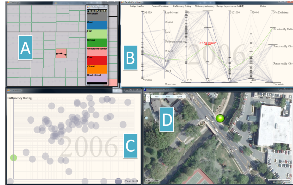
Figure 4: (A) A significant downward temporal trending indicates an unusual pattern (B) Using PCView to compare different structural attributes (C) Examining certain bridge on SPView, indicating this is the earliest constructed bridge in the database (D) The Geospatial view shows that this bridge is constructed on top of a river stream.
